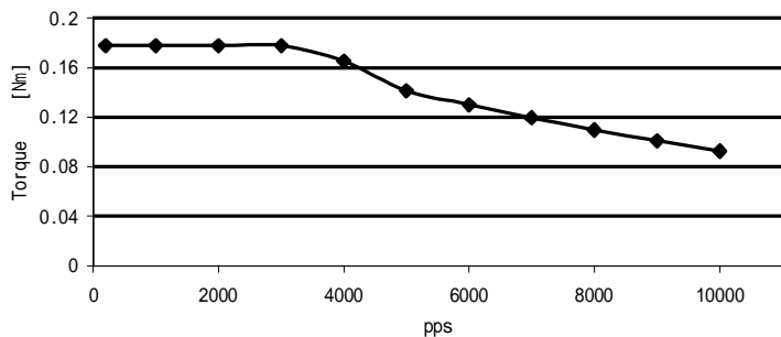
BL42STH33-0956A VM: 24VDC; 1A /相 驱动器: HA335, 半步
