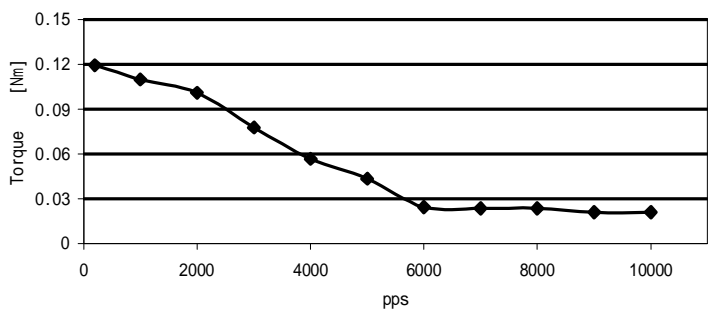
BL42STH33-0316A VM: 24VDC; 0.3A /相 驱动器: M415B, half step
