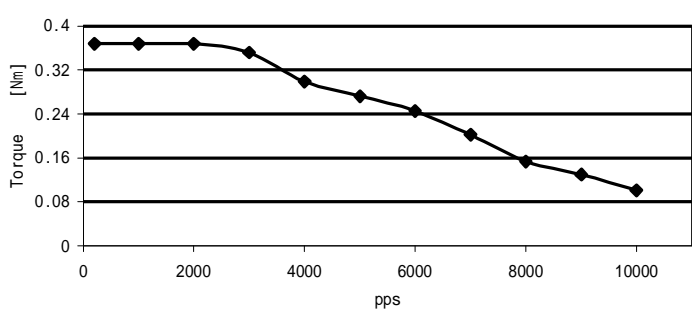
BL42STH38-1684A VM: 24VDC; 1.77A /相 驱动器: HA335, 半步
