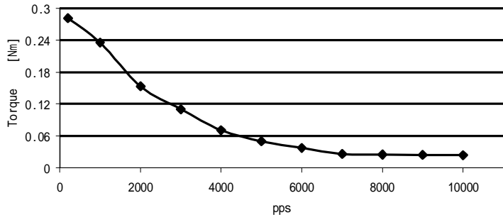
BL42STH38-0806A VM: 24VDC; 0.8A /相 驱动器: M325, 半步
