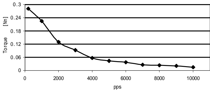
BL42STH33-0406A VM: 24VDC; 0.5A /相 驱动器: HA335, 半步
