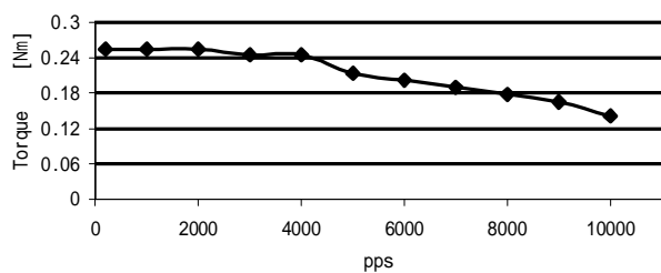
BL42STH33-1334A VM: 24VDC; 1.27A /相 驱动器: HA335, 半步
