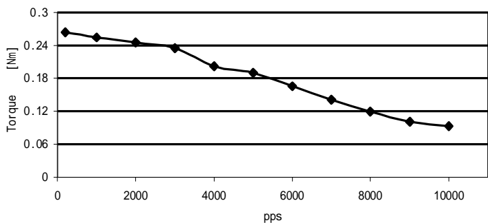
BL42STH38-1206A VM: 24VDC; 1.2A /相 驱动器: HA335, 半步
